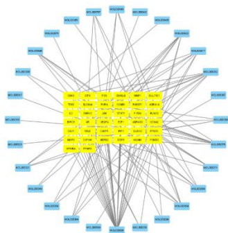
Figure 4. Disease-Compound-Target Network
