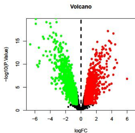
Figure 2. Volcano map
