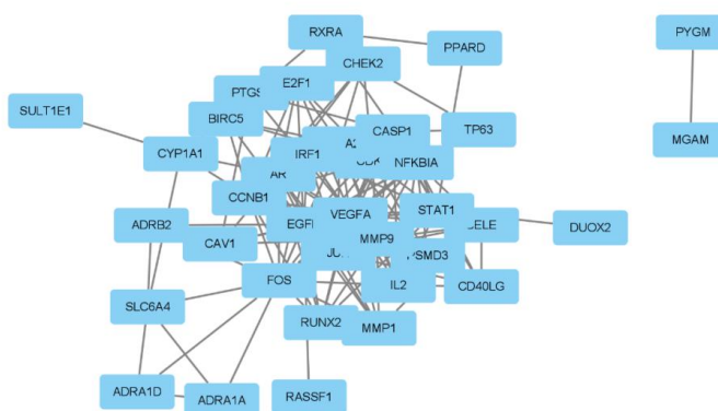
Figure 5. PPI network
